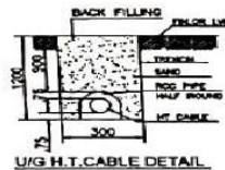
U/G H.T.CABLE DETAIL
